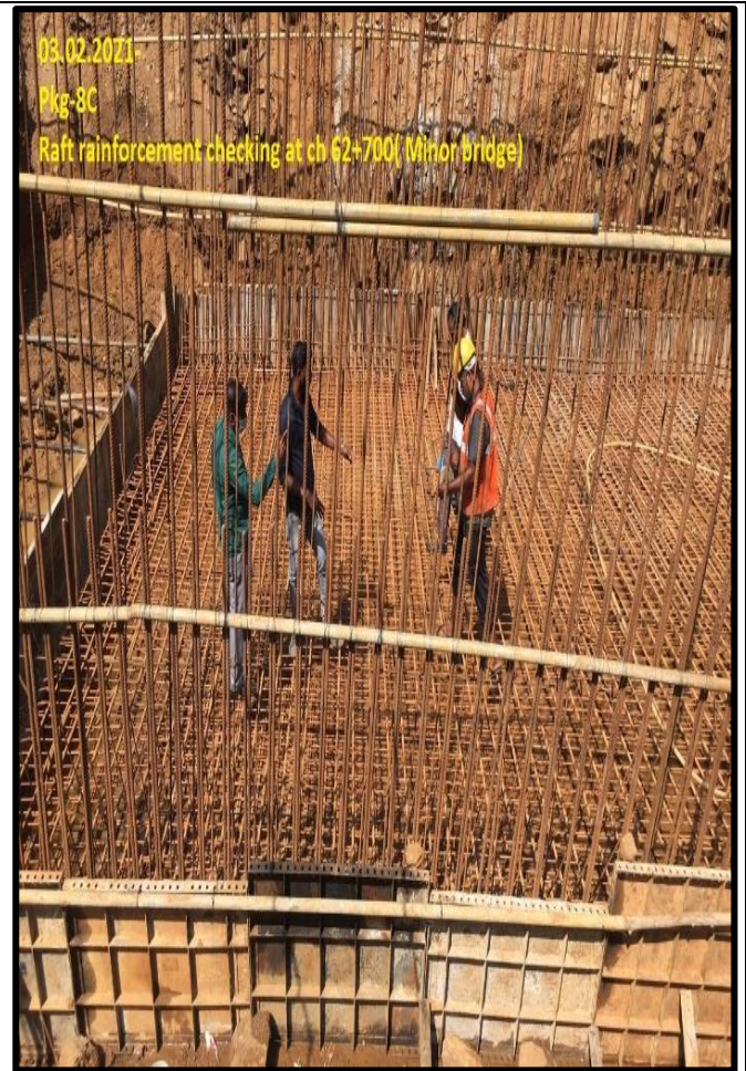
Raft reinforcement work in progress
