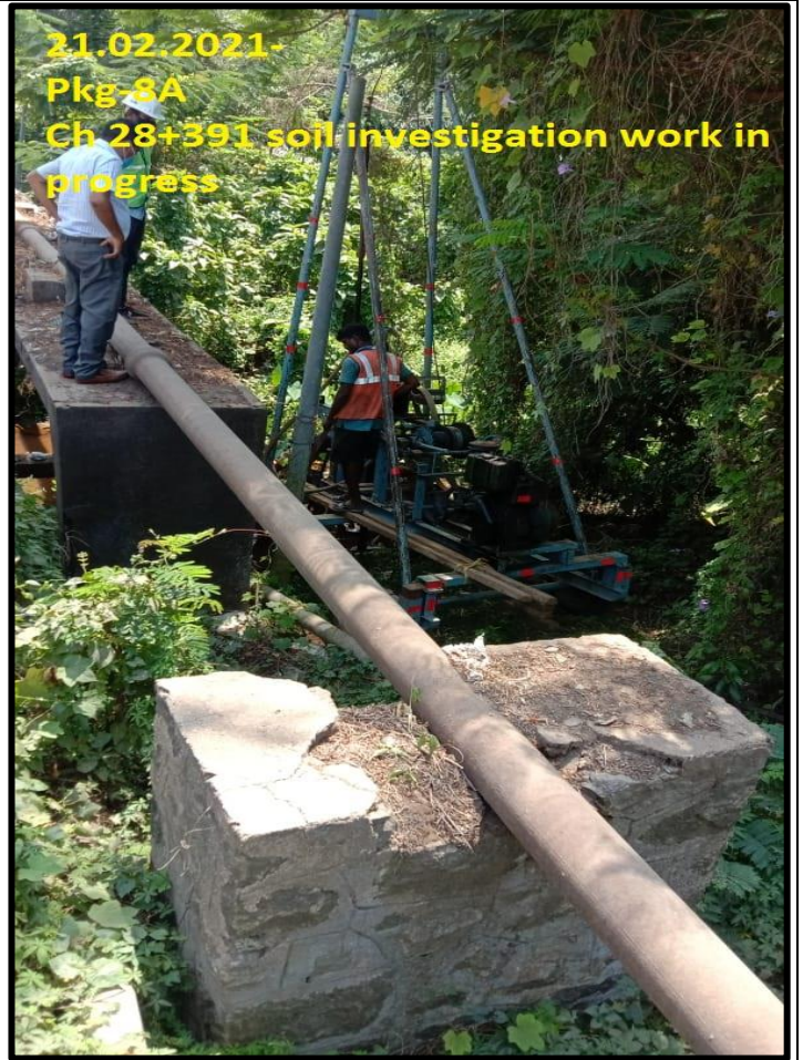
Soil investigation work in progress
