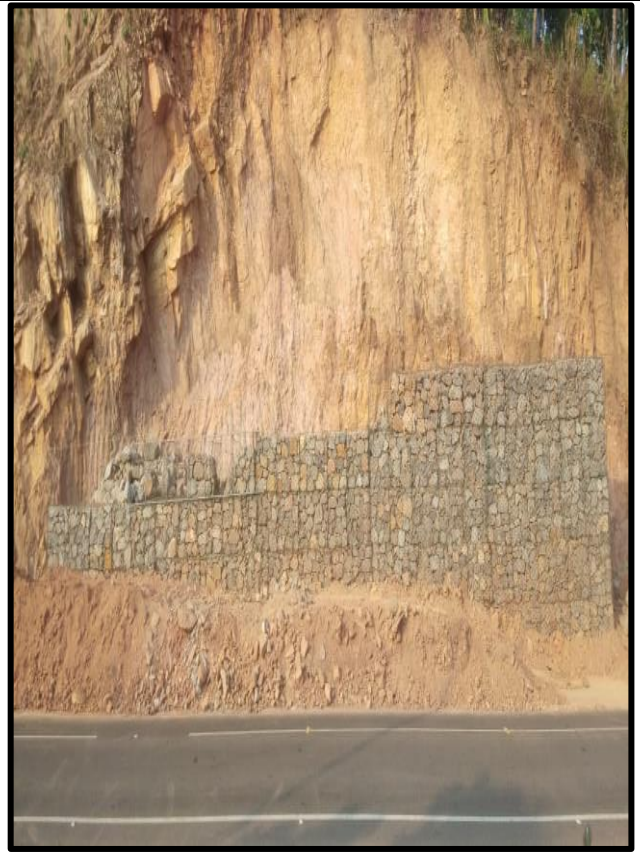
Gabion wall for hill protection work in progress at km 42+640 LHS.
