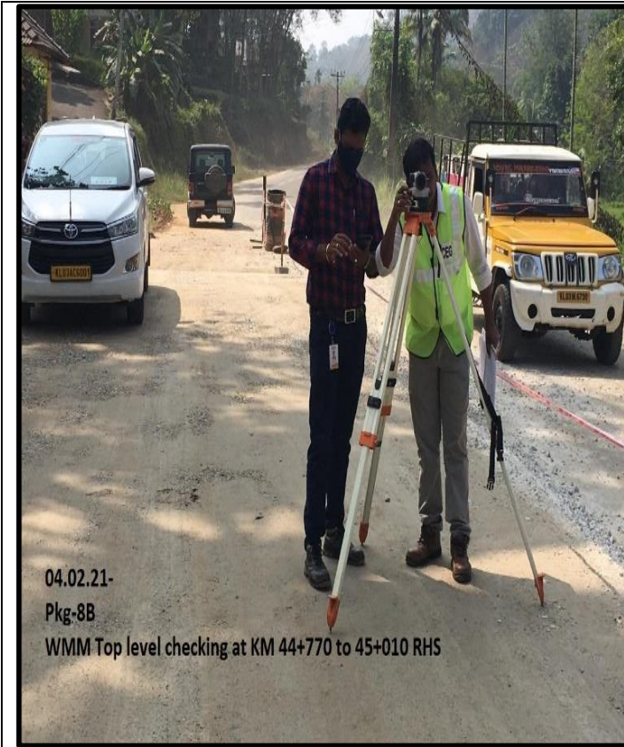
WMM Top level checking work in progress
