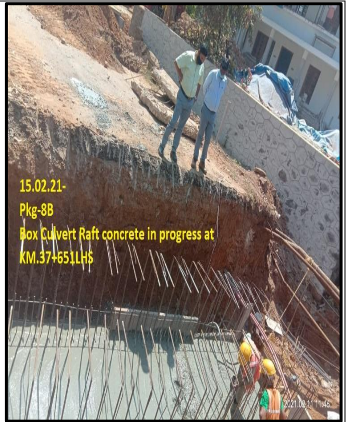
Box culvert Raft concrete work in progress
