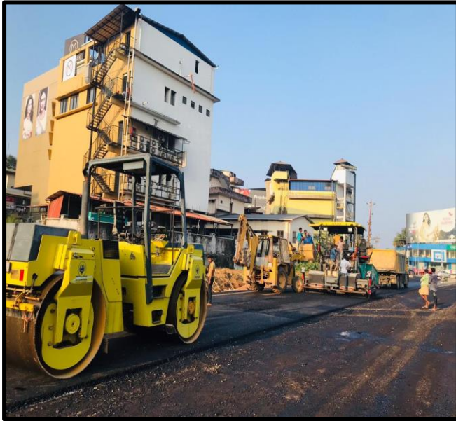
DBM work from Km:2+020 to Km:2+300
