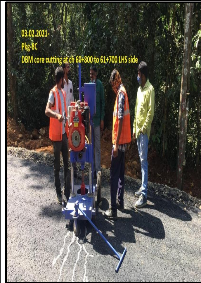
DBM core cutting at ch.60++800 to 61+700 LHS
