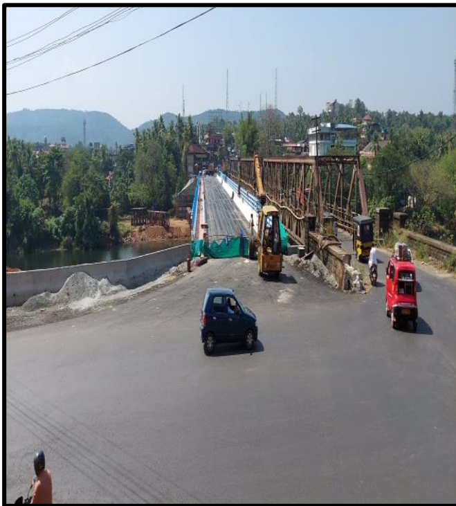
Bridge A2 side approach DBM Completed.
